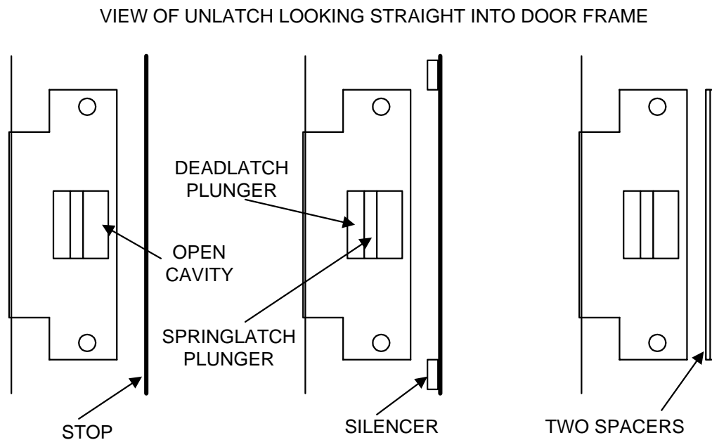
FIG. 4: FINAL ADJUSTMENT OF DOOR CLOSING TOLERANCE
